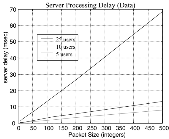
Figure 16. JASMINE server processing delay (data).
