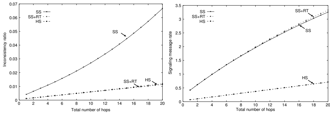
Figure 14: Inconsistency ratio and signaling message rate against total number of hops
