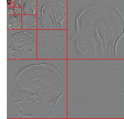
Wavelet-transformed, 5 iterations
