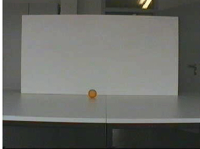
original image
