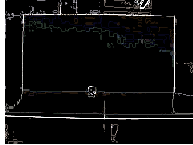
segmented image
