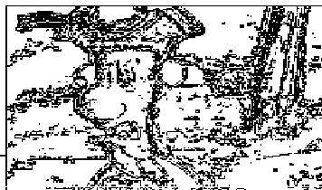
over-segmentation
