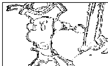
under-segmentation
