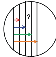
periodic structures
