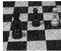
noisy image
