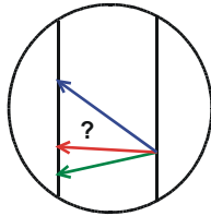
aperture problem
