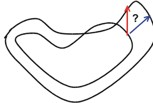
deformable objects
