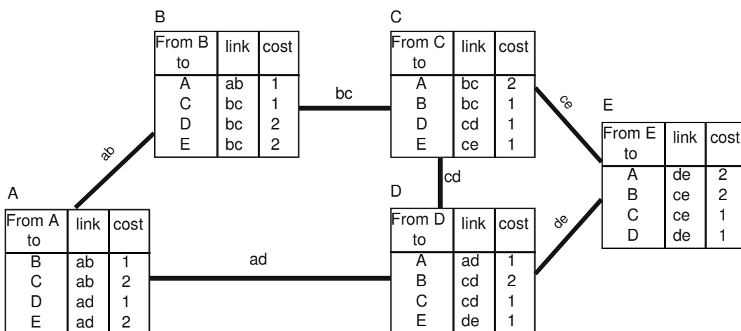
(b) after an exchange of RIP messages
