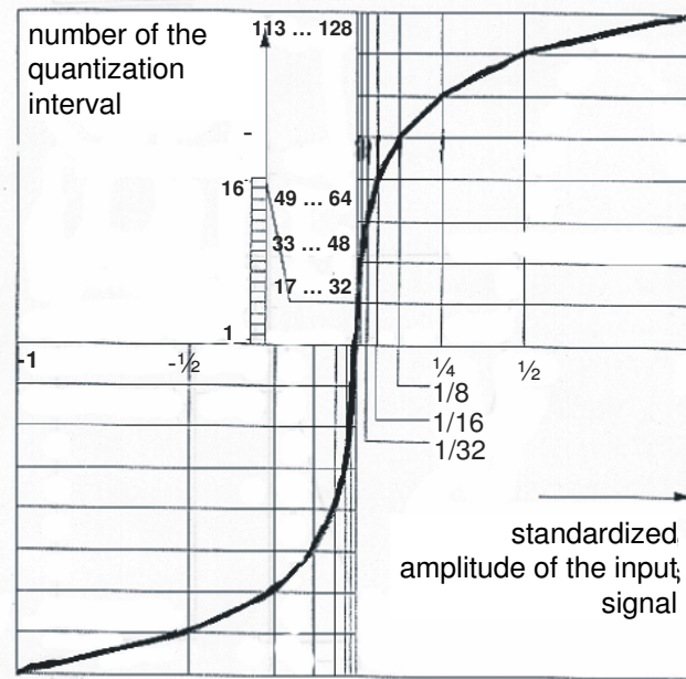
13-segment compressor curve
