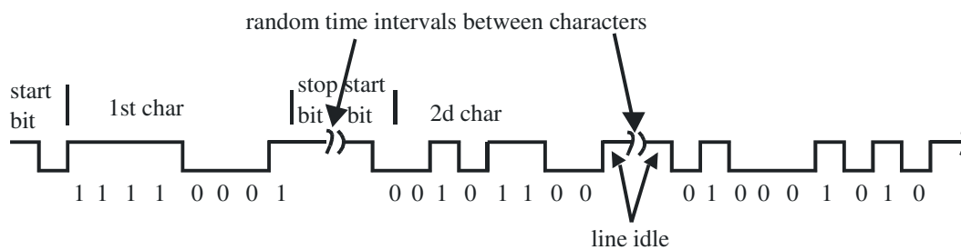
asynchronous bit stream
