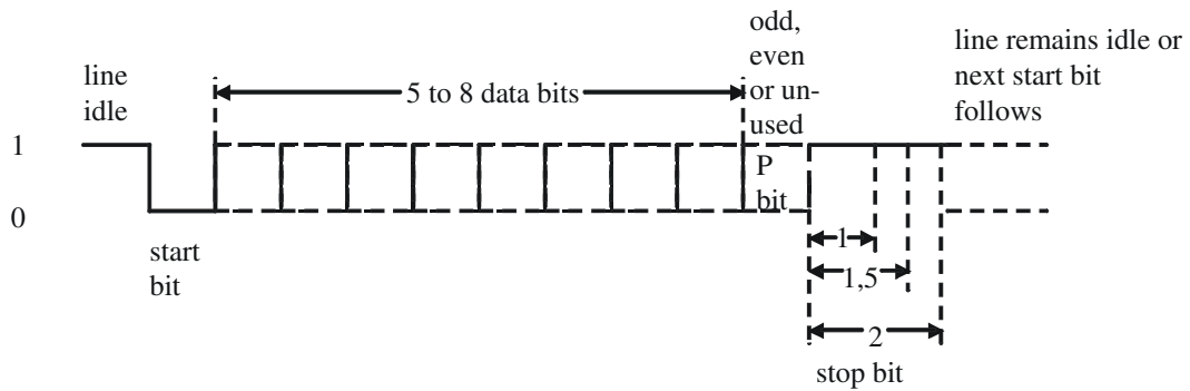
line coding for one character
