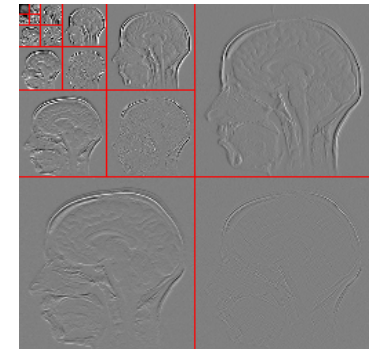
Wavelet-transformed, 5 iterations
