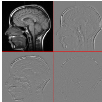
Wavelet-transformed, 1 iteration
