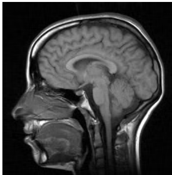
Original frame
