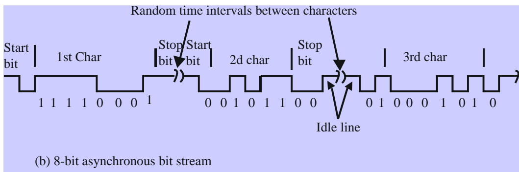
(b) Asynchroner Bitstrom
