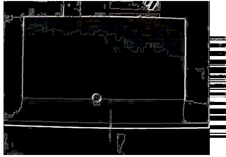
segmented image
