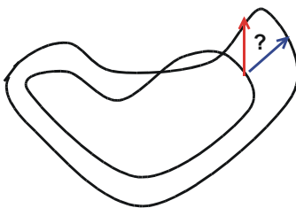
deformable objects
