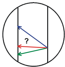
aperture problem
