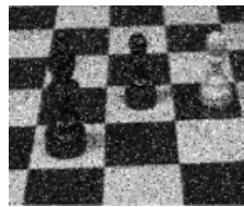
noisy image
