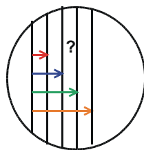
periodic structures
